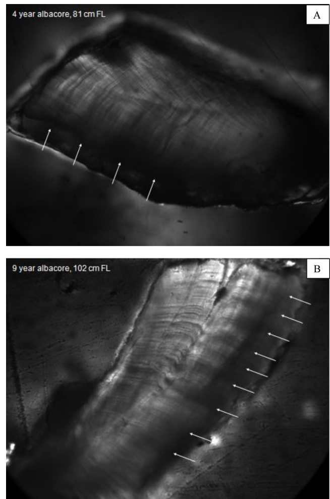
Fig. 4. Images of two North Pacific albacore sagittal otolith cross-sections estimated at (A) four years and (B) nine years of age.
